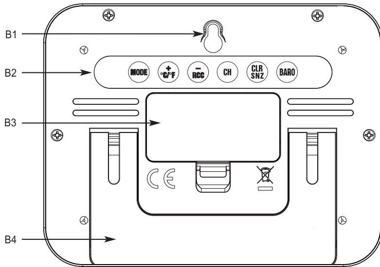
Fig. 2: Receiver
